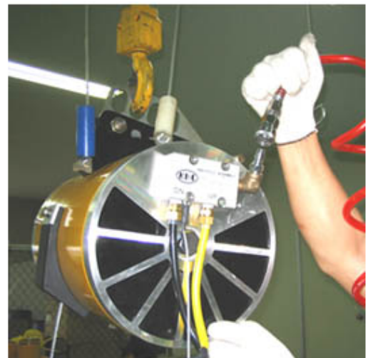
Air Hose Connection : 3/8 pt
