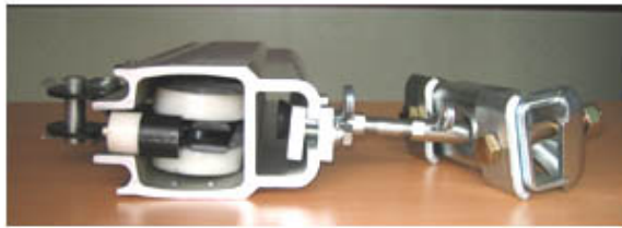
Trolley and Suspension Assy
